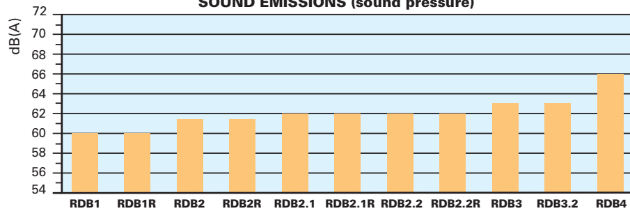
SOUND EMISSIONS (sound pressure)
